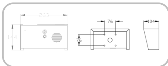
603-IMP-PED CALL PANEL
