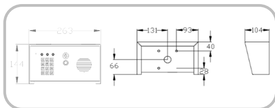
603-IMPK-PED CALL PANEL
